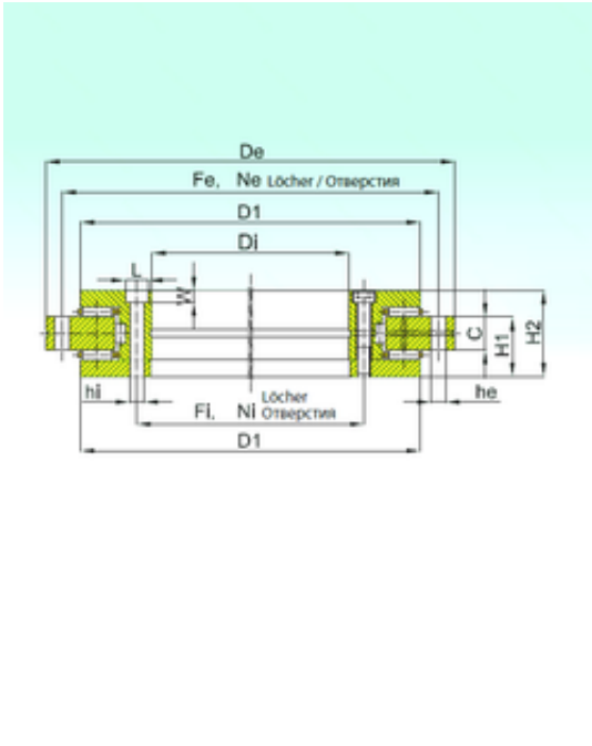
YRT 260 Bearing 2D drawings and 3D CAD models
